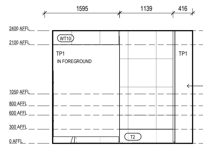
VILLAGE AMENITIES - MALE WC - 2
