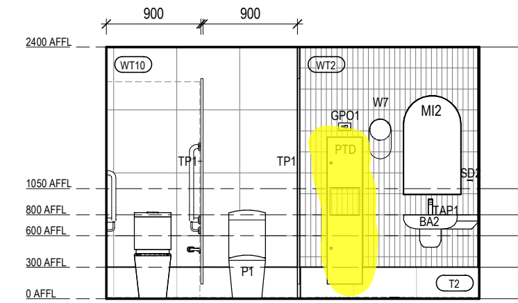
VILLAGE AMENITIES - FEMALE WC - 1
