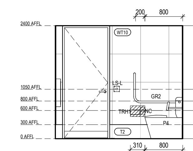
VILLAGE AMENITIES - ACC WC - 4
