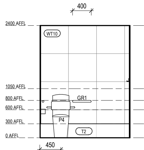
VILLAGE AMENITIES - ACC WC - 1
