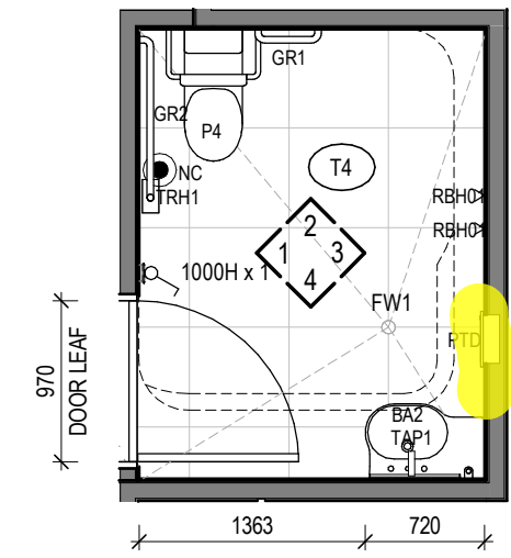
3 RACF AMENITIES - ACCESSIBLE WC 01 Scale 1: 50
