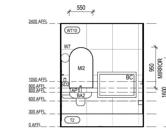
VILLAGE AMENITIES - ACC WC - 3
