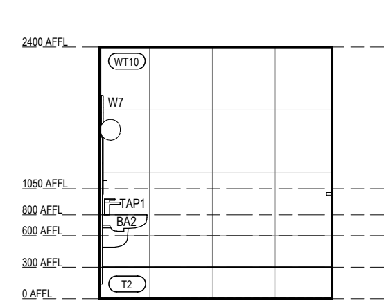
VILLAGE AMENITIES - FEMALE WC - 3
