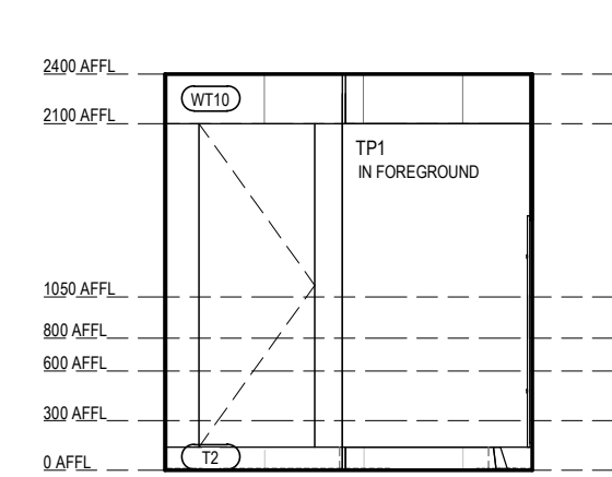
VILLAGE AMENITIES - FEMALE WC - 2
